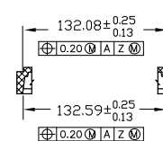
SECTION J-J
